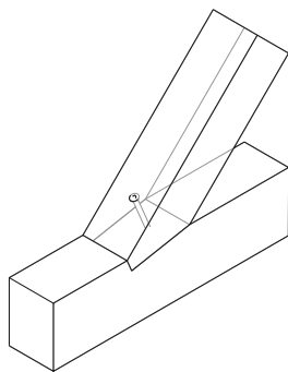
Single step joint
