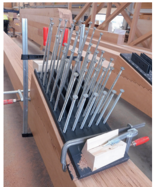
SWG production hall – Lattice girders connection with 12 mm full thread screws
