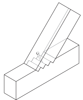
Multiple step joint
